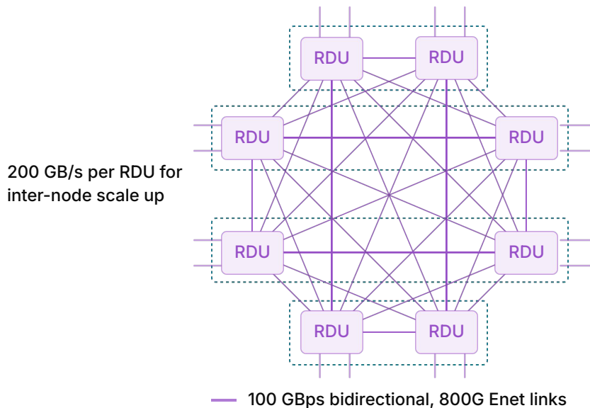
8-socket Node: Scale-Up Topology
