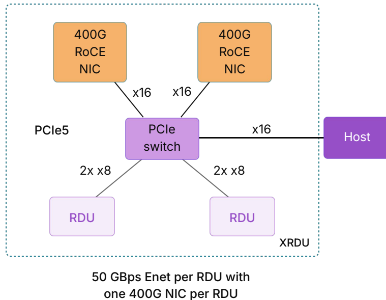
8-socket Node: 1 Scale-Out NIC per RDU
